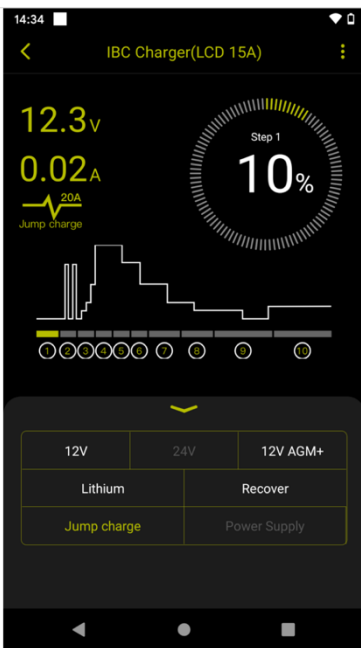
Power-Button and overview of the charging parameters
