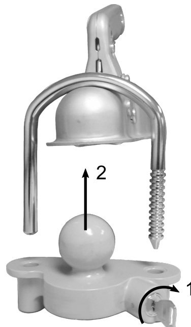
Figure 3: Inserting into the coupling claw
